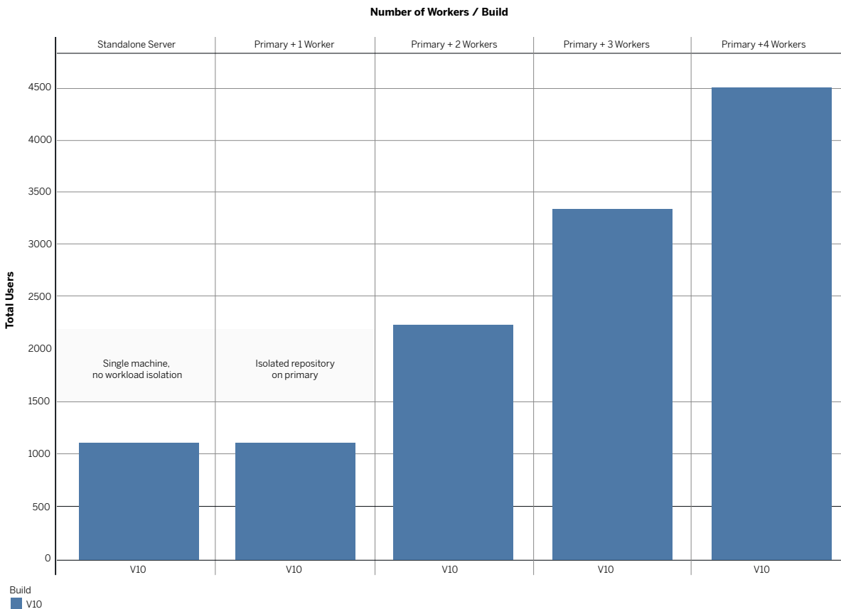
Figure 7: Tableau Server scalability (total users) scales linearly with more workers.
