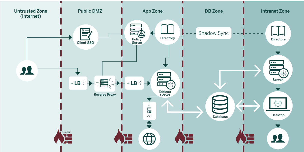
Figure 6: An overview enterprise-class deployment
